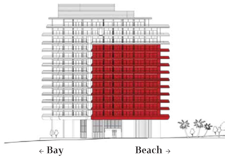
SOUTH FACADE
